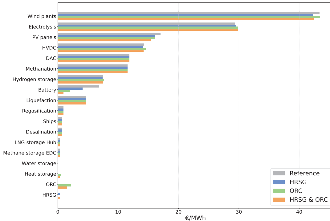
Figure 4: Breakdown of costs per scenario and technology
