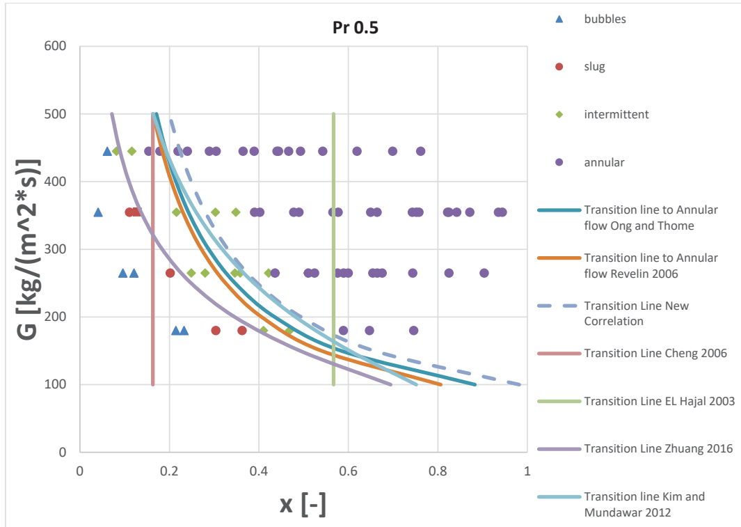
Figure 14. Flow map for reduced pressure 0.5
