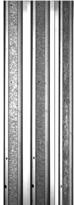
Figure 7. Flow Patterns Pr=0,8 G=355 kg/(m 2 ·s) Quality respectively: 8.2%, 19%, 33,7%.
