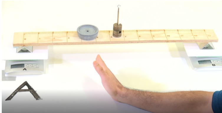
Figure 1: Snapshot of a sample hands-on activity to find beam support reactions.
